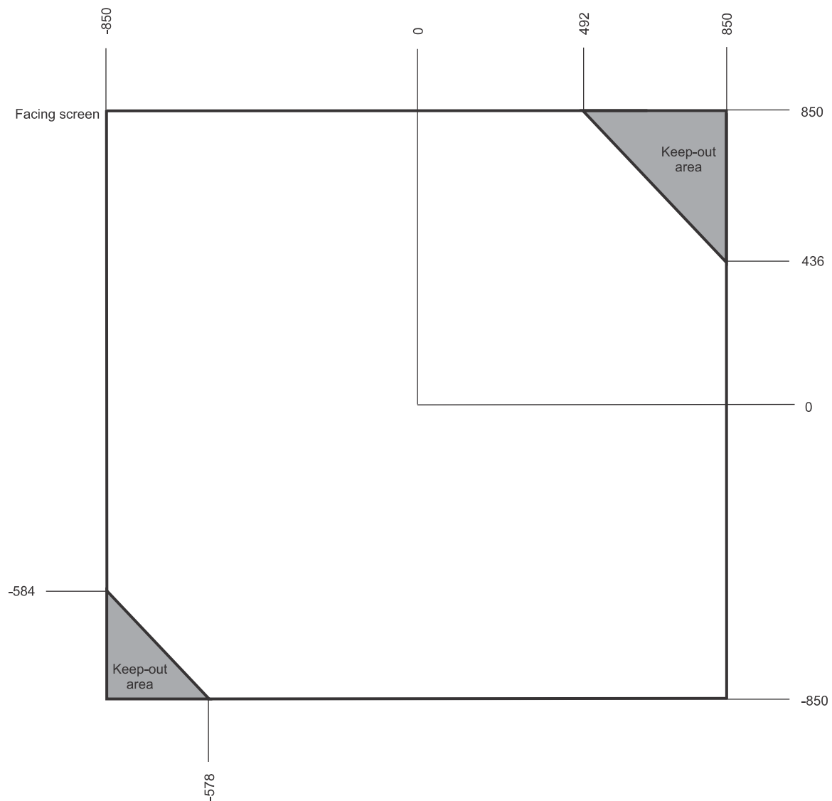
Christie M 4K RGB series lens keep-out zones
